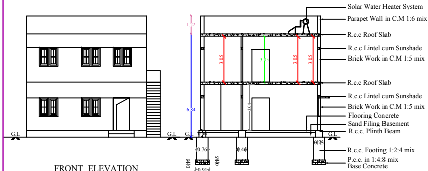
FRONT ELEVATION
