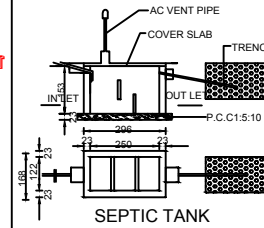
SEPTIC TANK
