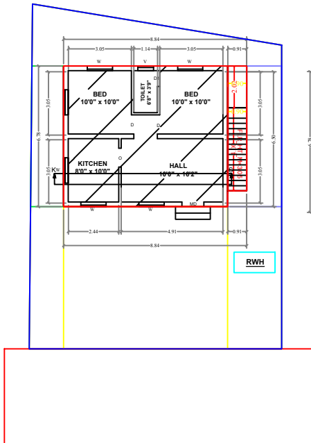
EXG.GROUND FLOOR PLAN
