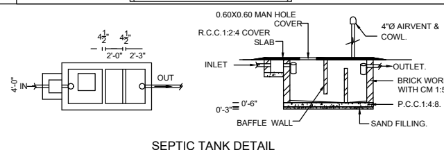
SEPTIC TANK DETAIL
