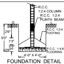
FOUNDATION DETAIL
