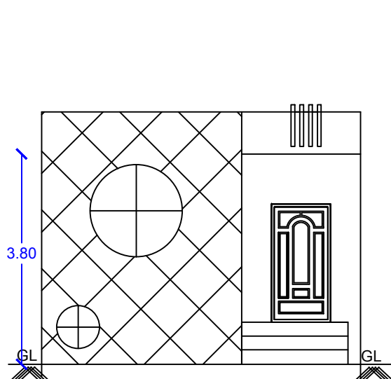
FRONT ELEVATION (EAST FACING)
