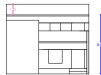
ELEVATION FACING EAST
