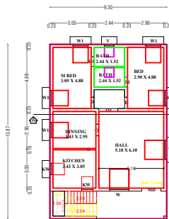
GROUND FLOOR FACING EAST
