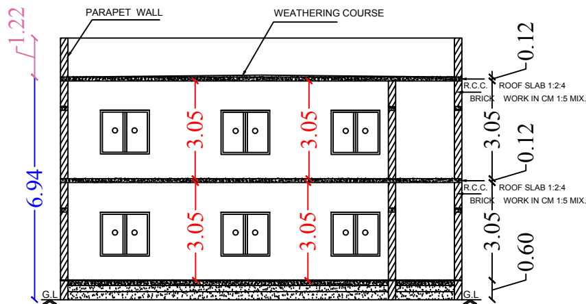
Section on-"AA"
