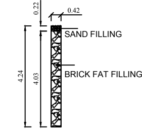
DETAILS OF PERCULATION PIT
