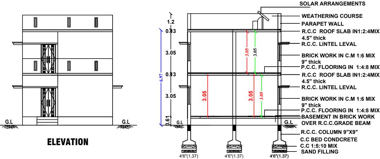
SECTION " AB "
