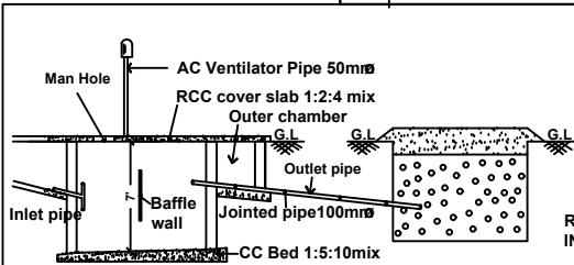
SECTION FOR SEPTIC TANK AND D.T (NOT TO SCALE)
