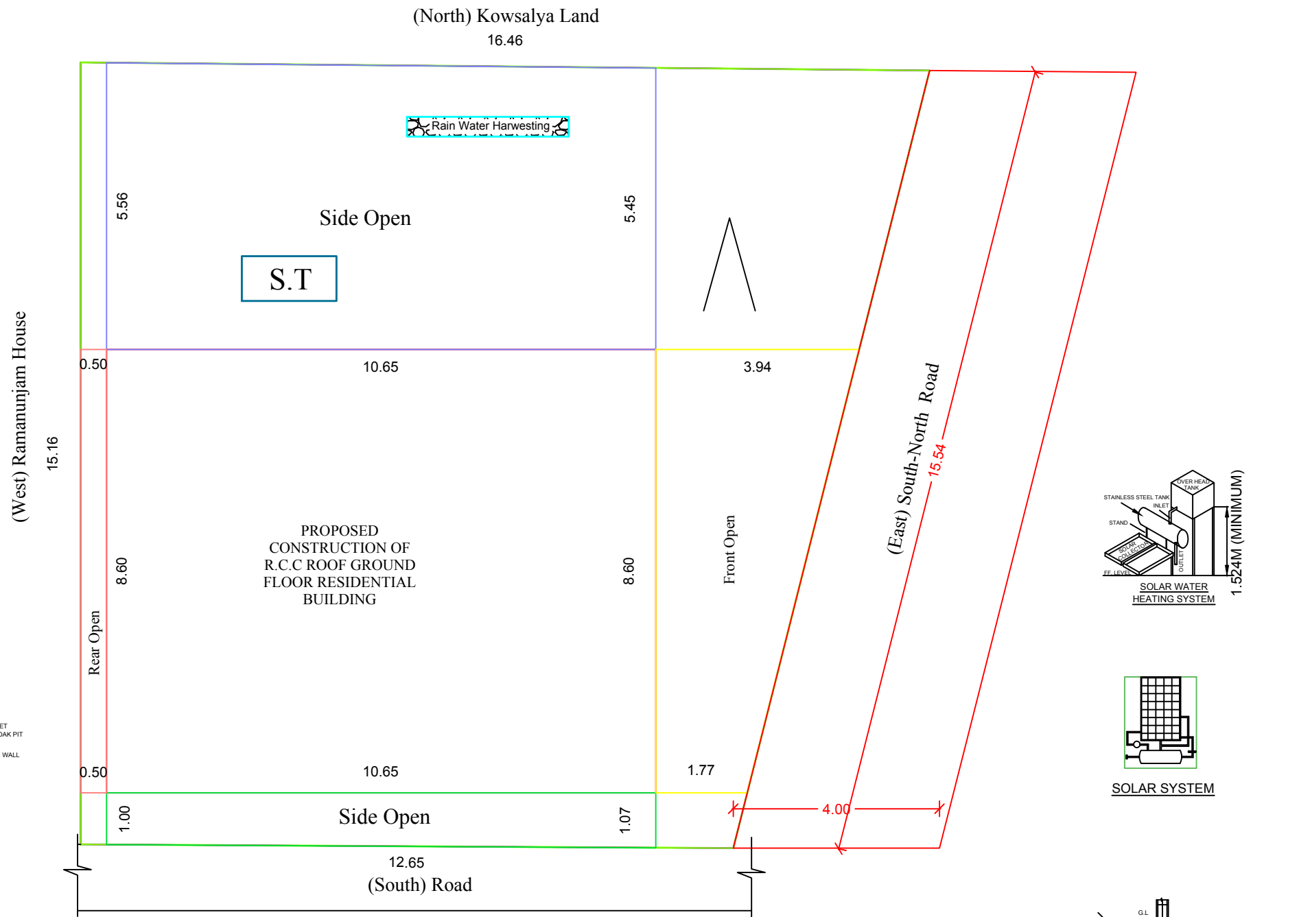
SITE PLAN
