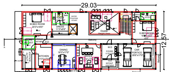
PROPOSED GROUND FLOOR PLAN
