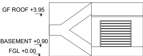
FRONT ELEVATION
