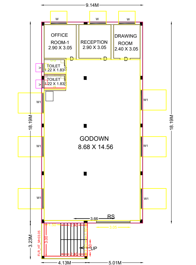
PROPOSED GODOWN FLOOR PLAN (EAST FACING)
