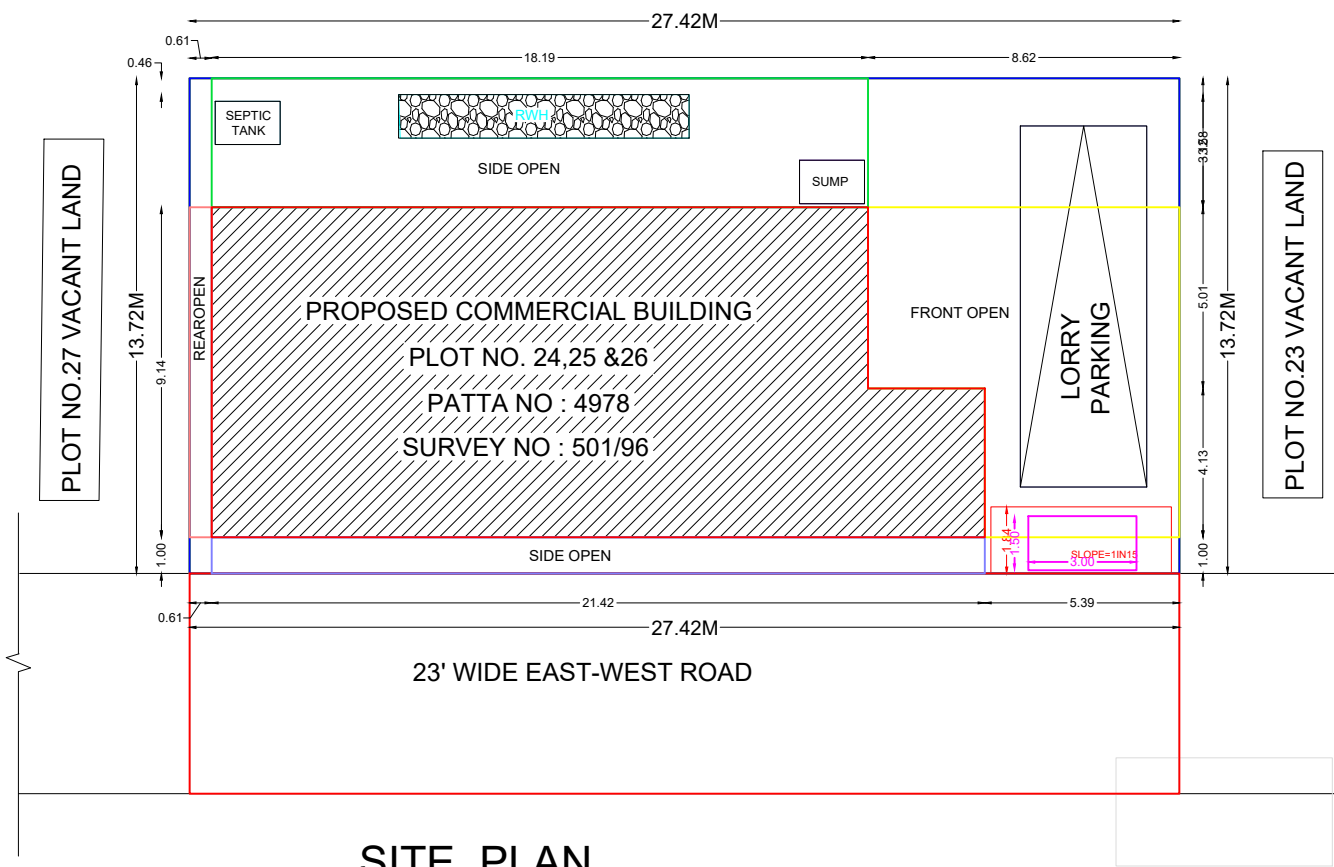
SITE PLAN
