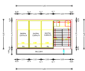
PRO. FIRST FLOOR PLAN (COMMERCIAL)
