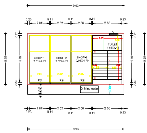
PRO. GROUND FLOOR PLAN (COMMERCIAL)
