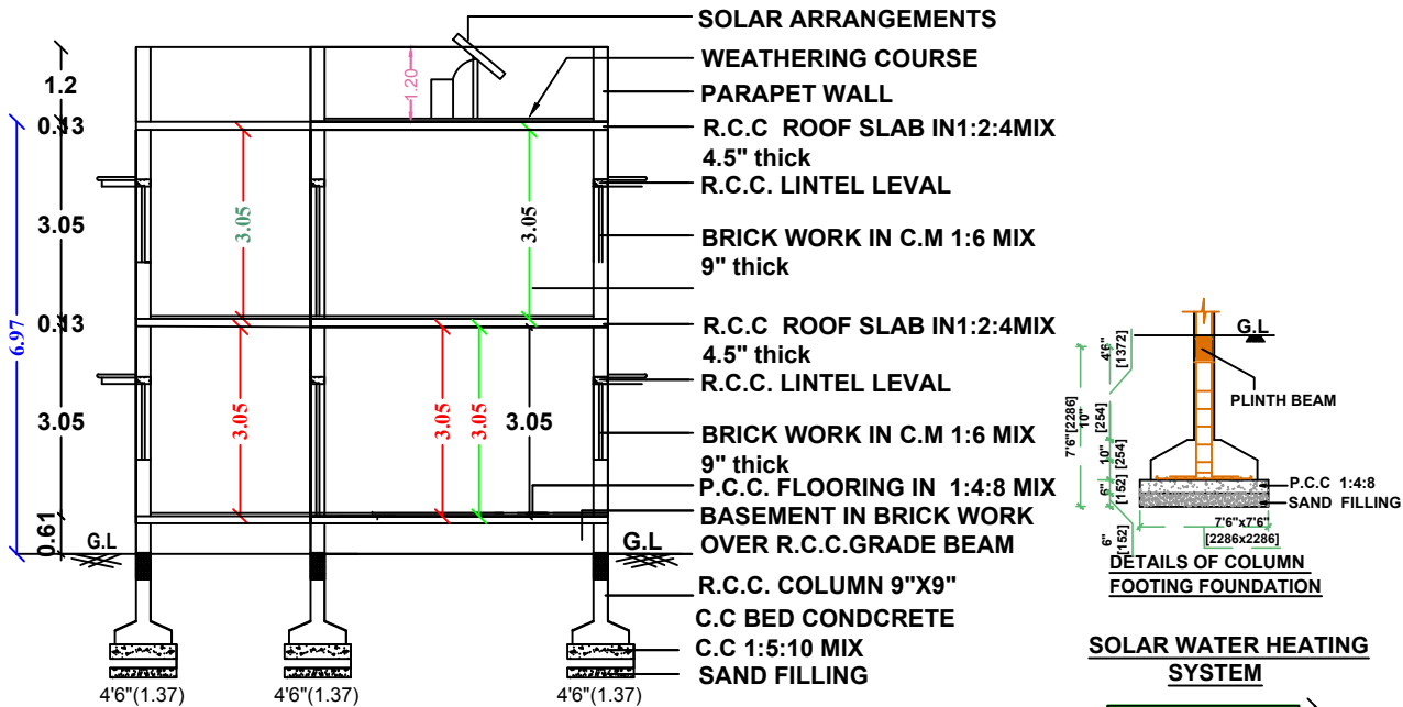
SECTION " AB "
