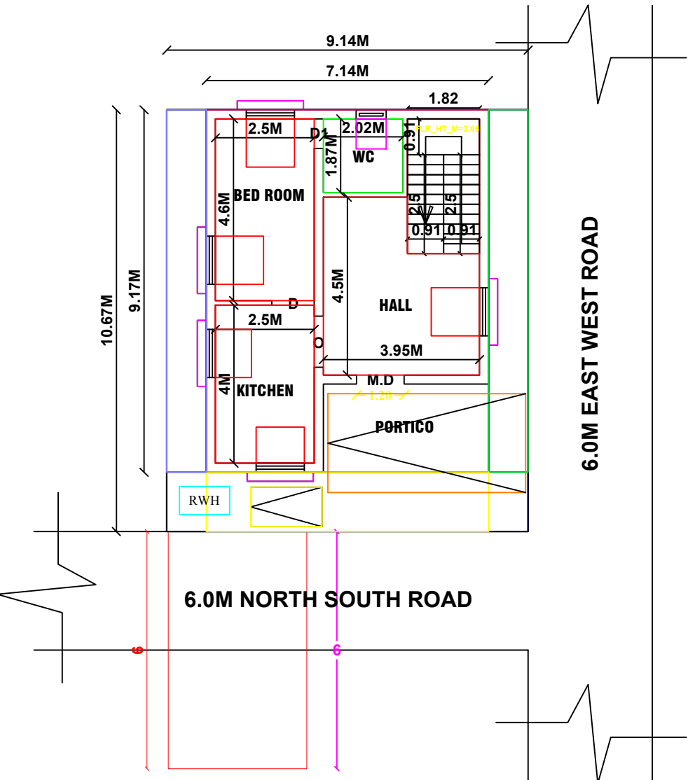
GROUND FLOOR
