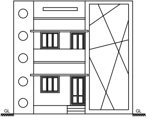
FRONT ELEVATION
