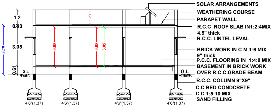
SECTION " AB "
