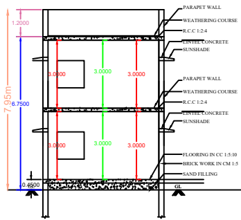
SECTION AB
