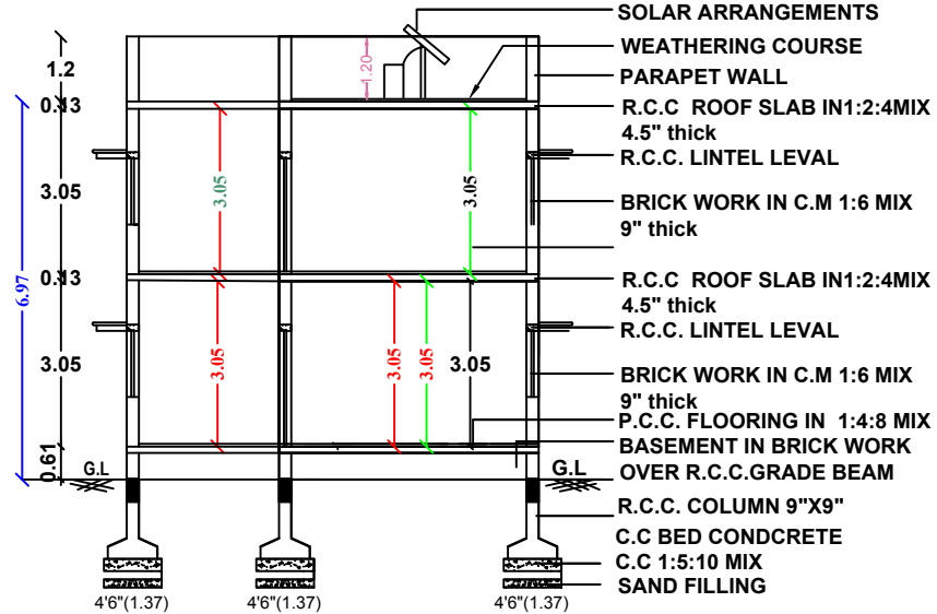
SECTION " AB "
