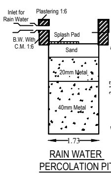
RAIN WATER PERCOLATION PIT
