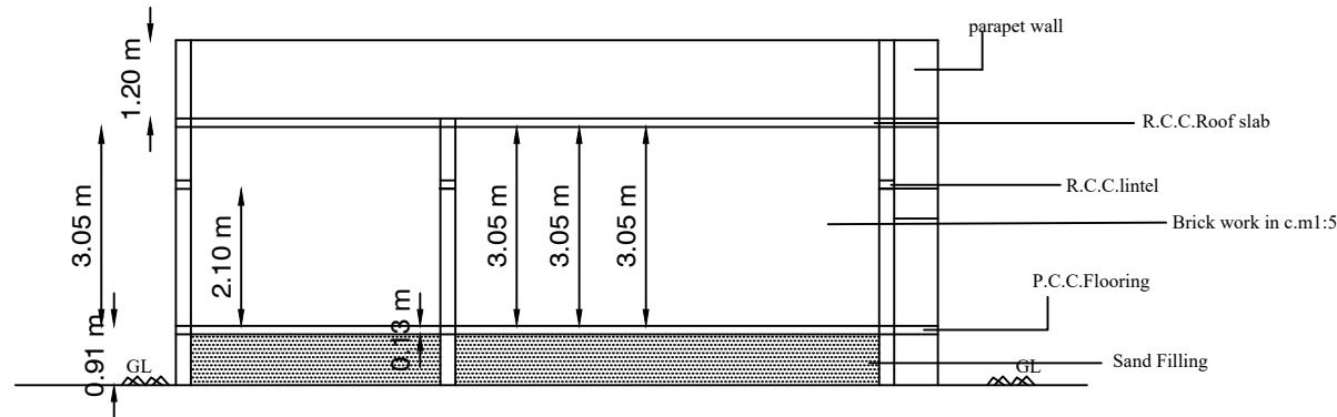
SECTION-"SR"
