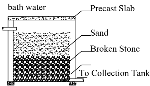
Section of Filter Unit
