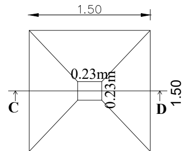
SECTION - 'CD'
