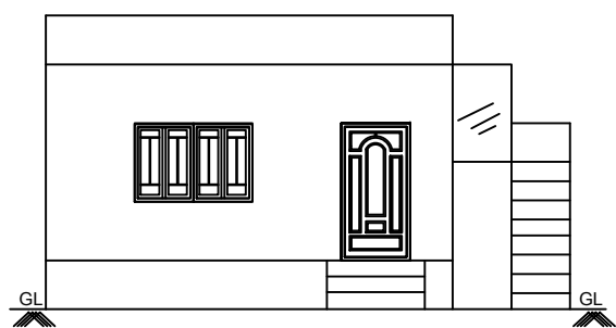
FRONT ELEVATION (EAST FACING)
