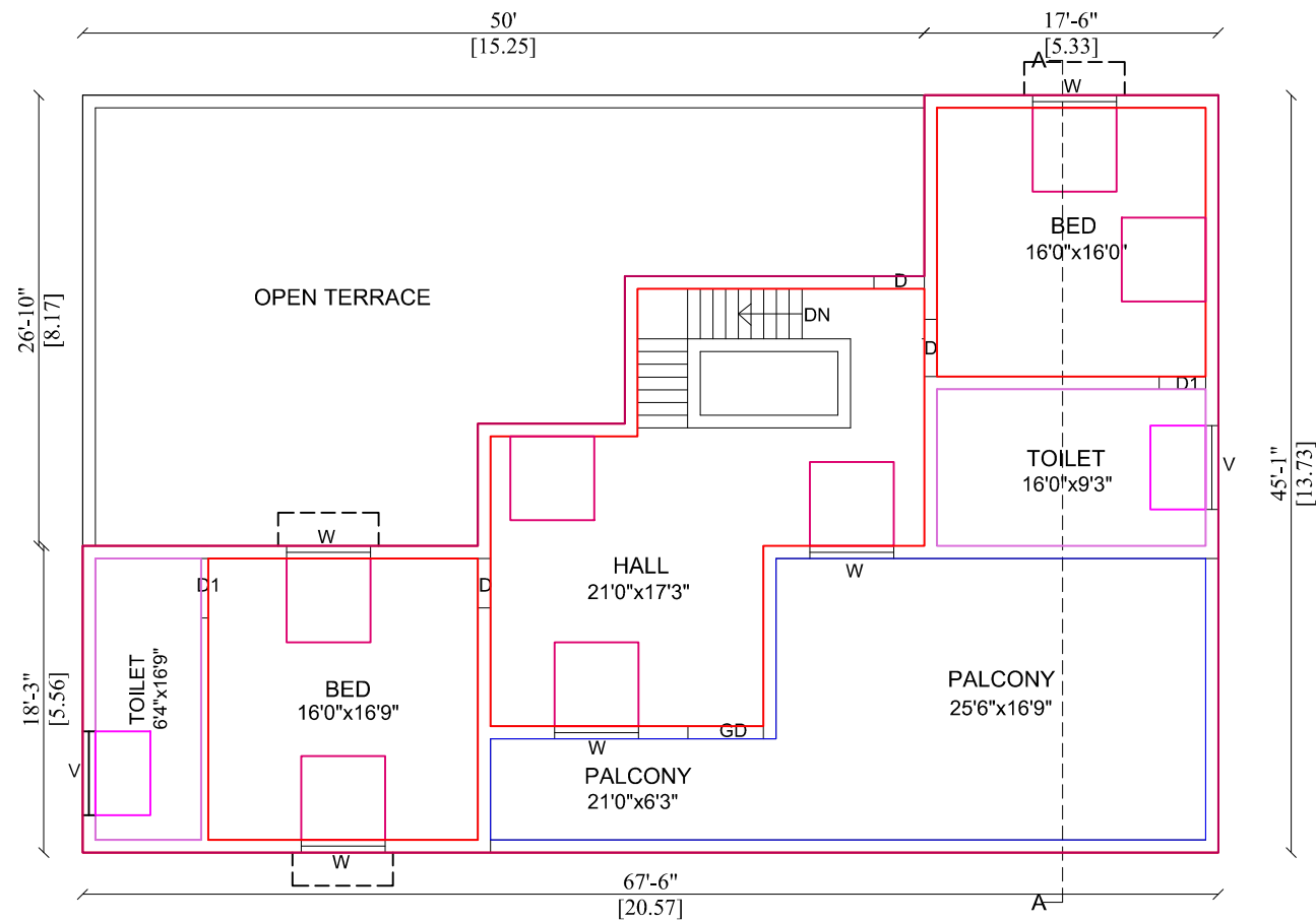
PRO.,FIRST FLOOR PLAN
