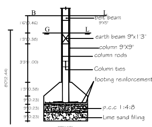
FOUNDATION DETAILS
