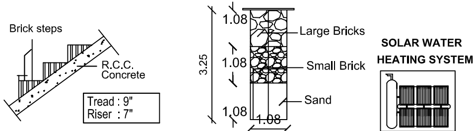
STAIRCASE DETAILS
