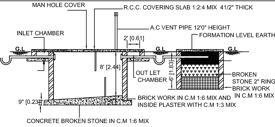
SECTION OF SEPTIC TANK AND DISPERSION TRENCH
