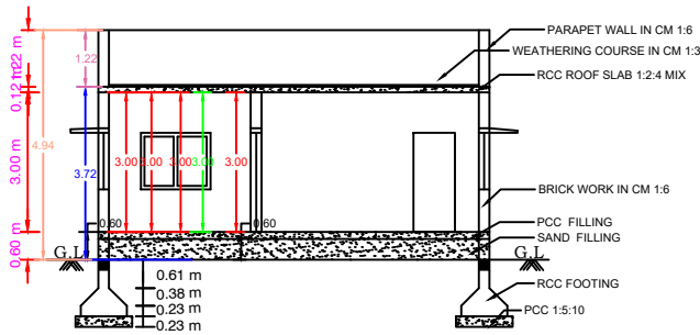
SECTION OF KA
