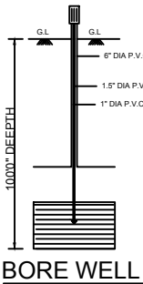
BORE WELL
