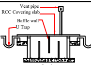
Waste Water Recycle Unit
