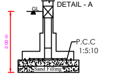
FOUNDATION DETAIL - A
