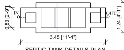
SEPTIC TANK DETAILS-PLAN
