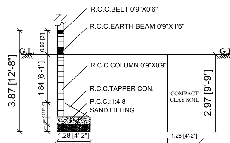
FOUNDATION DETAILS-END COLUMN
