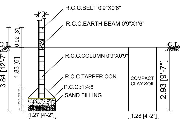
FOUNDATION DETAILS-MIDDLE COLUMN
