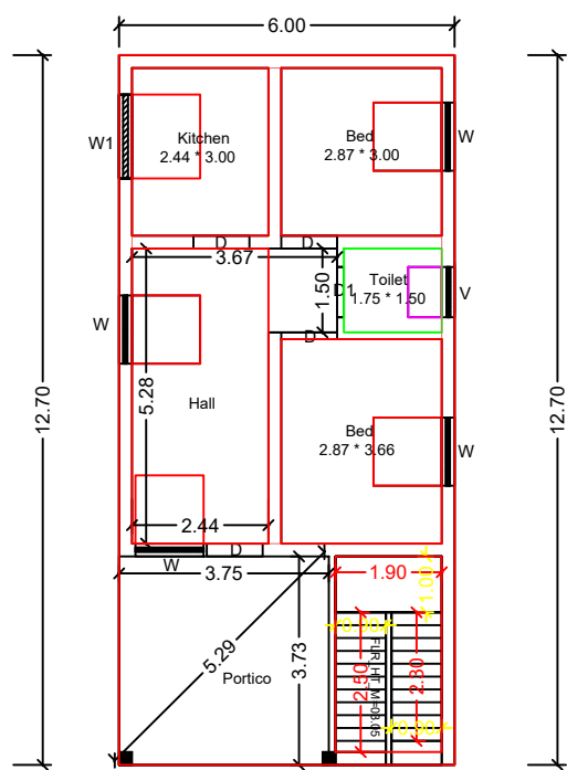
PLAN -Demolished & Additional Ground Floor
