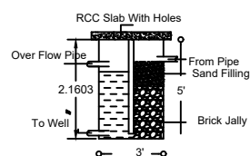
RWHS Tank Details
