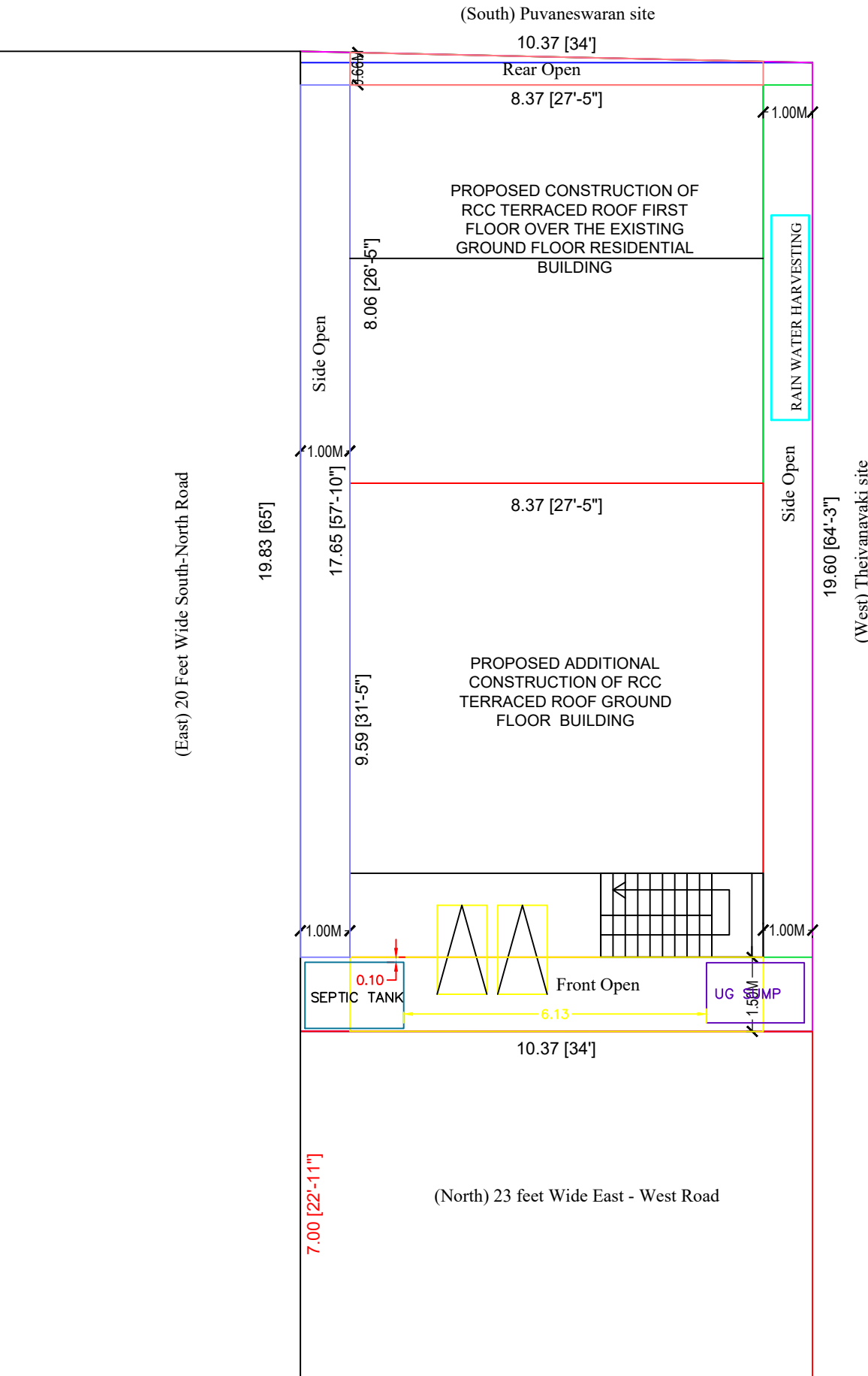
SITE PLAN
