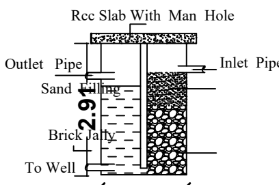
RWHTank Details
