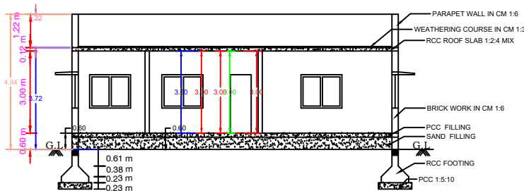
SECTION OF KA
