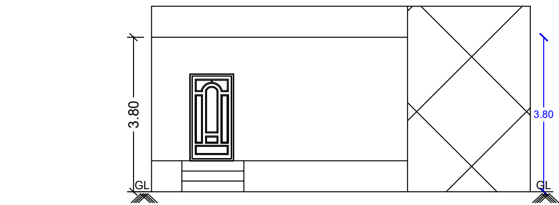
FRONT ELEVATION (NORTH FACING)
