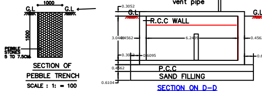
SECTION ON D-D
