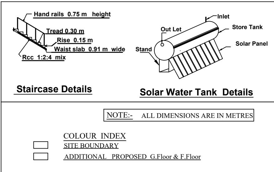
DEMOLISED & ADDITIONAL PROPOSED
