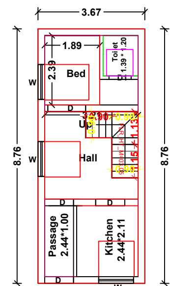
DEMOLISED & ADDITIONAL PROPOSED
