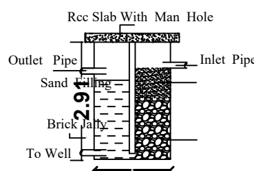
RWHTank Details
