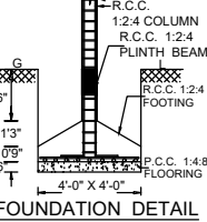
FOUNDATION DETAIL
