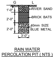
RAIN WATER PERCOLATION PIT (NTS)
