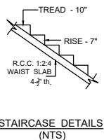
STAIRCASE DETAILS (NTS)
