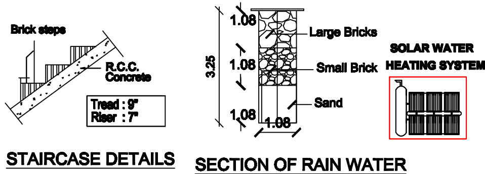
SECTION OF RAIN WATER
