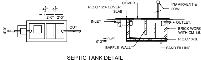
SEPTIC TANK DETAIL
