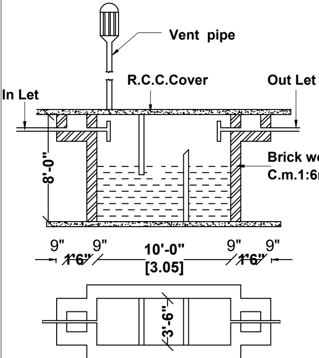
SEPTIC TANK DETAILS (NOT TO SCALE)
