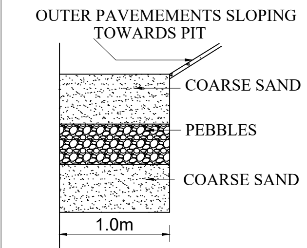
RAIN WATER PERCOLATION BED
