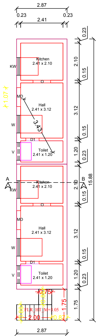
PRO.GROUND FLOOR PLAN
