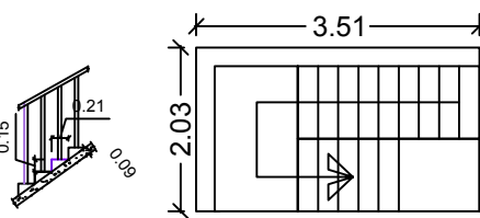
STAIRCASE DETAILS
