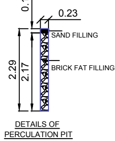
DETAILS OF PERCOLATION PIT
