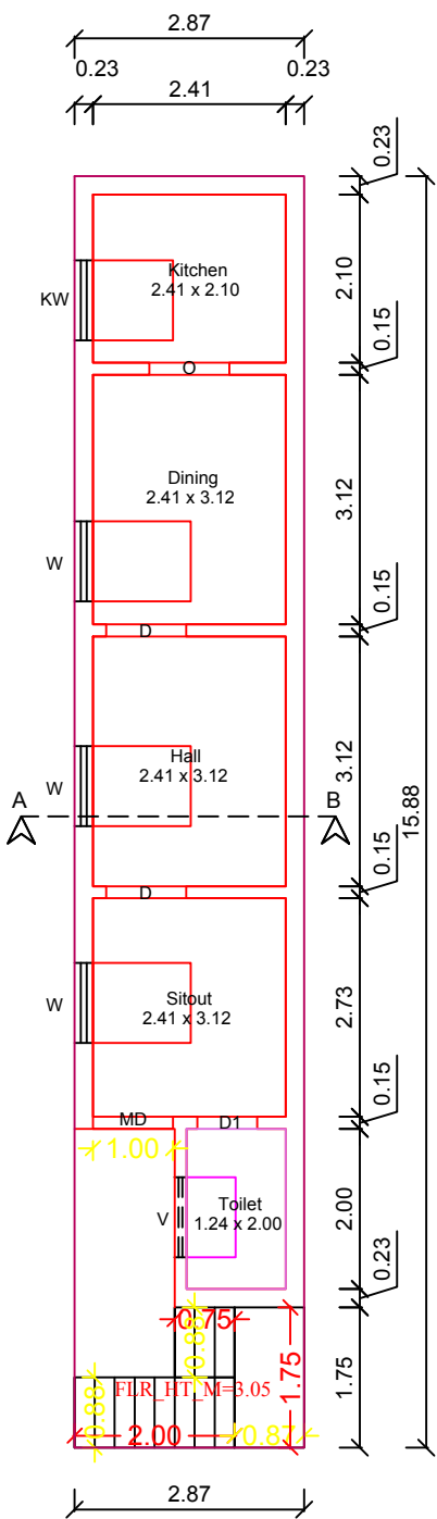
PRO.FIRST FLOOR PLAN
