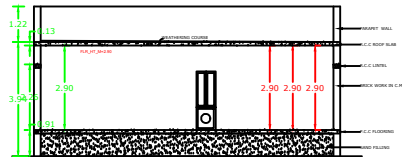
SECTION ON K-S
