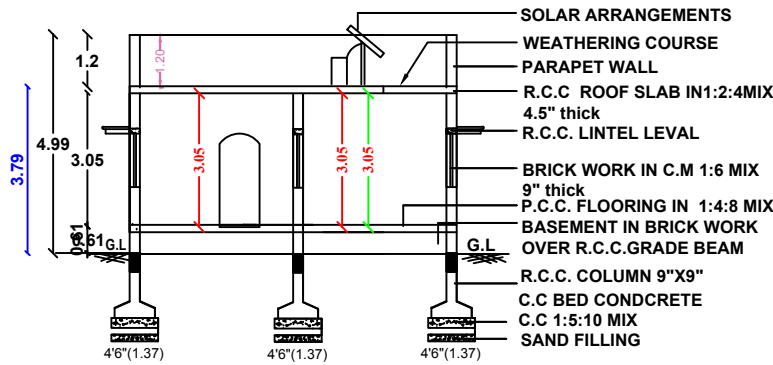
SECTION " AB "
