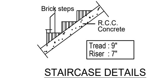
STAIRCASE DETAILS
