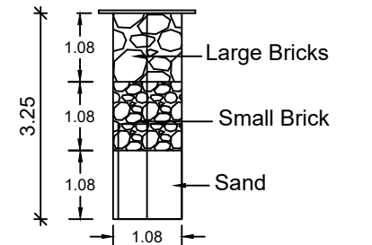
SECTION OF RAIN WATER COLLECTION PITS (NTS)
