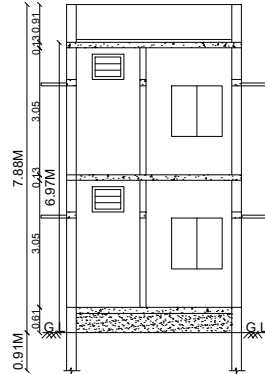
SECTION ON "BK"
