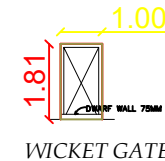
WICKET GATE
