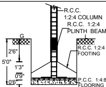
FOUNDATION DETAIL
