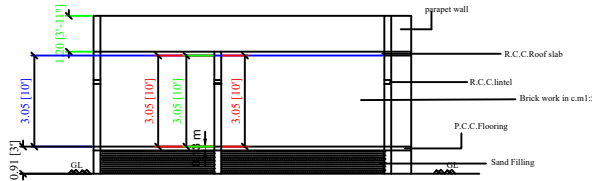
SECTION-"SR"
