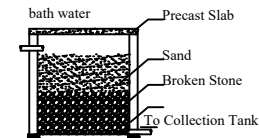
Section of Filter Unit
