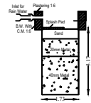
RAIN WATER PERCOLATION PIT
