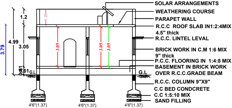
SECTION " AB "
