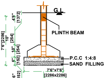
DETAILS OF COLUMN FOOTING FOUNDATION
