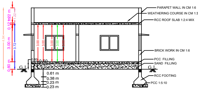
SECTION OF KA
