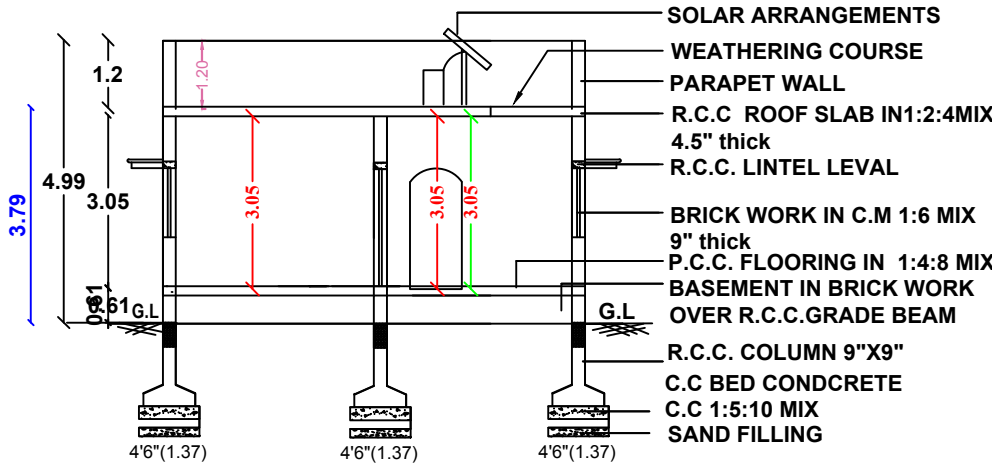
SECTION " AB "
