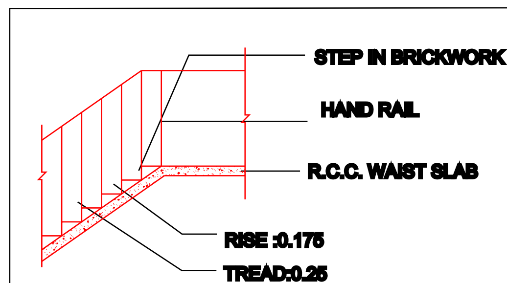
STAIR DETAILS
