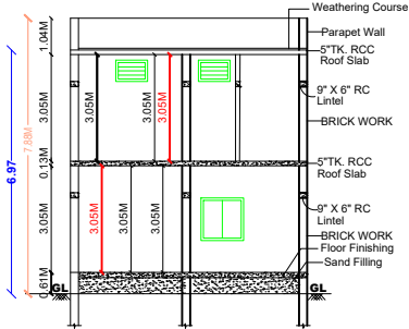
SECTION-"SR"
