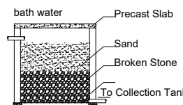
Section of Filter Unit
