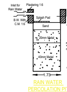
RAIN WATER PERCOLATION PIT
