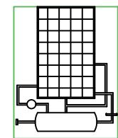
SOLAR SYSTEM
