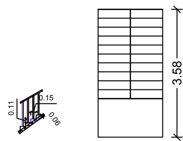
STAIRCASE DETAILS
