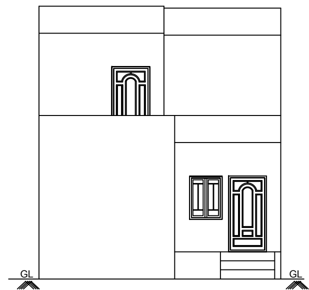
FRONT ELEVATION (EAST FACING)
