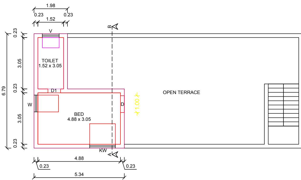
PRO.FIRST FLOOR PLAN
