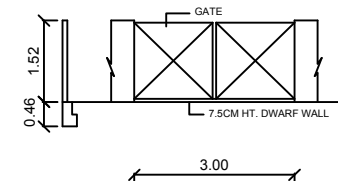
COMPOUND WALL WITH DWARF WALL DETAILS
