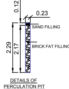
DETAILS OF PERCOLATION PIT
