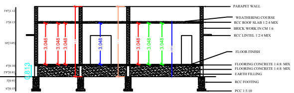
SECTION ON 'XX'
