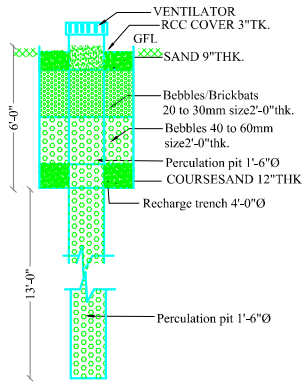
RAIN WATER STORAGE SCALE: 1"=4'-0"
